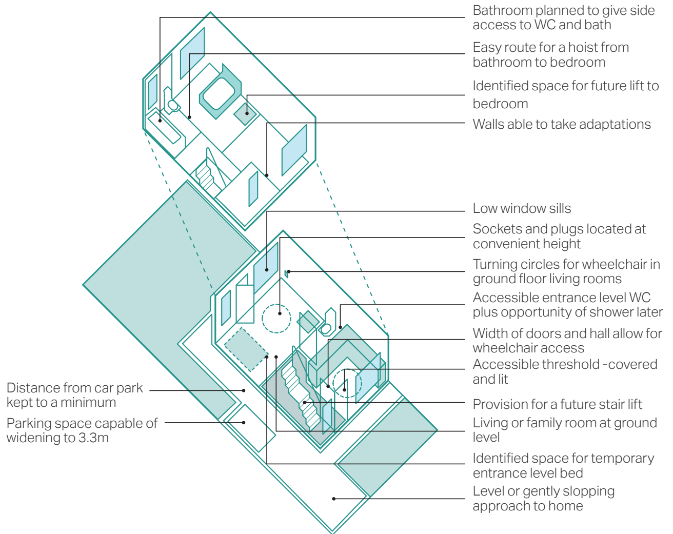
Figure 117: Diagram to illustrate the main principles of inclusivity, accessibility, adaptability and sustainability.
